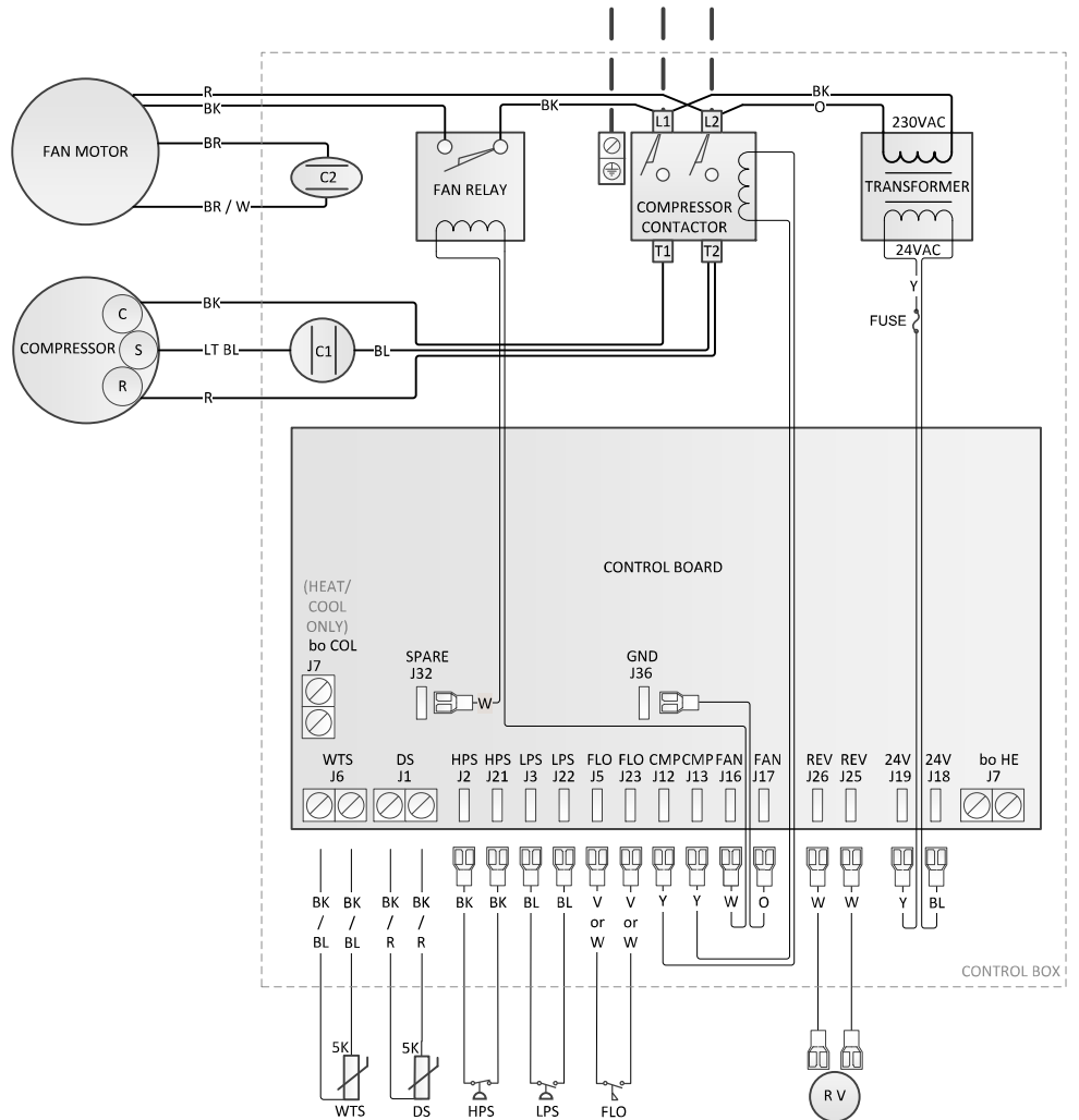
FIGURE 4: 240 VAC / 60 Hz Singe Phase Wiring Diagram
