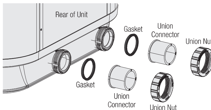
FIGURE 9: Included Union Connectors
