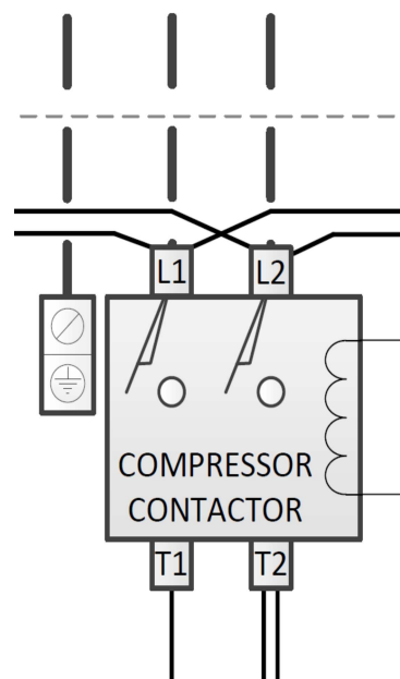
FIGURE 13: Power Connections
