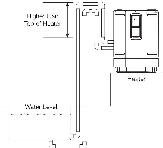
FIGURE 10: Heater Installation Above Pool
